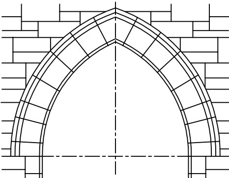
Gothic
